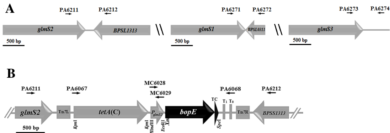
Figure 5.1.4 Primers used for confirmation of the site of genomic integration of pUC18Tmini-Tn7T:: tetA(C)::P glmS2 ::bopETC . (A) Schematic representation of the wild-type gene glmS2 ( BPSL1312 ) and its adjacent gene BPSL1313 , glmS1 ( BPSL0312 ) and its adjacent gene BPSL0311 , and glmS3 . The primer pairs PA6211/PA6212, PA6271/PA6272 and PA6273/6274 were used to identify if there was an insertion after glmS2 , glmS1 and glmS3 , respectively. (B) Schematic representation of the wild-type glmS2 and BPSL1313 after the expected integration of pUC18Tmini-Tn7T:: tetA(C)::P glmS2 ::bopETC construct into the chromosome. The primer pair combinations PA6067/MC6029, MC6028/PA6068 and MC6028/PA6212 were used for further analyses. The following features are indicated: Tn7L and Tn7R, left and right end of Tn7; tetA(C) , tetracycline resistance cassette cloned at the KpnI site; P glmS2 , glmS2 promoter derived from the wild-type strain and cloned at HindIII (5') and EcoRI (3'); bopE , full length bopE derived from the wild-type strain and cloned at XmaI (5') and SpeI (3') sites; TC, tetracycline tag cloned at the SpeI site; T 1 T 0 , transcriptional terminators T 1 and T 0 from bacteriophage \lambda and E. coli rrnB operon, respectively. Arrows indicate the orientation of primers. Arrows designating oligonucleotides are not shown to scale.
