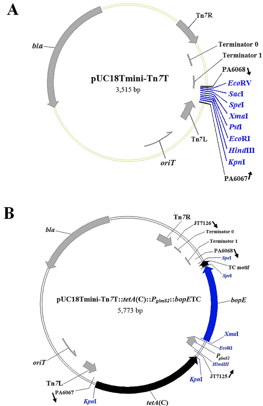
Figure 5.1.1 Plasmid maps of the empty pUC18T-miniTn7T vector (A) and the TC-tagged bopE construct in pUC18T-miniTn7T (B). The primer pair PA6067 and PA6068, amplifying a fragment containing the MCS of the plasmid, was used for verification of gene insertion and nucleotide sequencing. The following features are indicated: Tn7L and Tn7R, left and right end of Tn7, respectively; tetA(C) , tetracycline resistance cassette derived from pUTminiTn5Tc vector and cloned into the KpnI site; P glmS2 , glmS2 promoter derived from the wild-type strain and cloned at the HindIII (5') and EcoRI (3') sites; bopE , full length bopE derived from the wild-type K96243 strain and cloned at the XmaI (5') and SpeI (3') sites; TC motif, tetracycline motif cloned at a SpeI site; oriT , origin of conjugative transfer; T 1 T 0 , transcriptional terminators T 1 and T 0 from bacteriophage \lambda and E. coli rrnB operon, respectively. Arrows indicate gene orientation.
