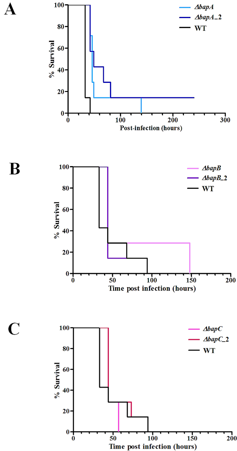
Figure 3.8.4 Kaplan-Meier survival curves of BALB/c mice infected intranasally with 10^7 CFU of the K96243 AbapA (A), AbapB (B), AbapC (C) or the wild-type strain. There was a significant difference in the time to death for mice infected with the bapA mutant and the K96243 AbapA_2 strains in comparison to the wild-type with ( P < 0.05 ). Mice infected with other mutants showed no difference in the time to death compared to mice infected the wild-type ( P > 0.05 ). AbapA denotes the K96243 AbapA strain; AbapA_2 denotes the K96243 AbapA_2 strain; AbapB denotes the K96243 AbapB strain; AbapB_2 denotes the K96243 AbapB_2 strain; AbapC denotes the K96243 AbapC strain; AbapC_2 denotes the K96243 AbapC_2 strain; WT denotes the wild-type strain.
